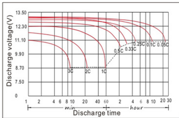
Discharge characteristic
