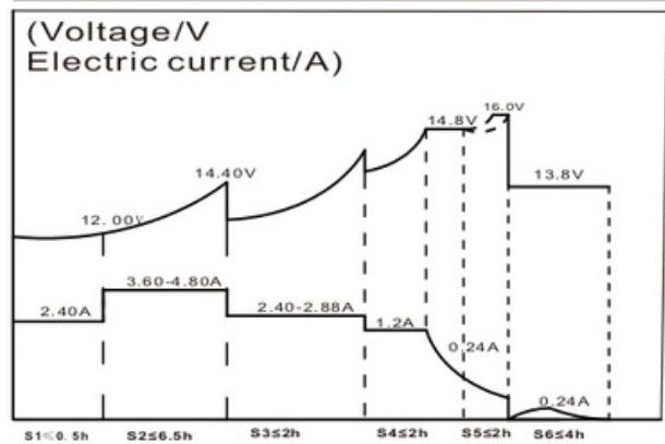
Charging characteristic
